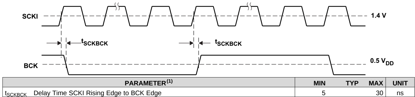
Figure 47. Audio Data Interface Timing (Master Mode: LRCK and BCK work as outputs)
