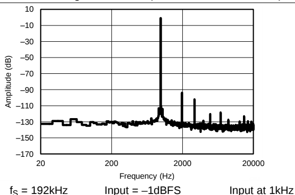
Figure 11. FFT with -1dBFS input
