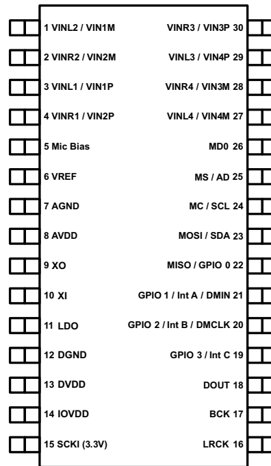
Figure 2. Device Pin Assignments, PCM1862, PCM1864
