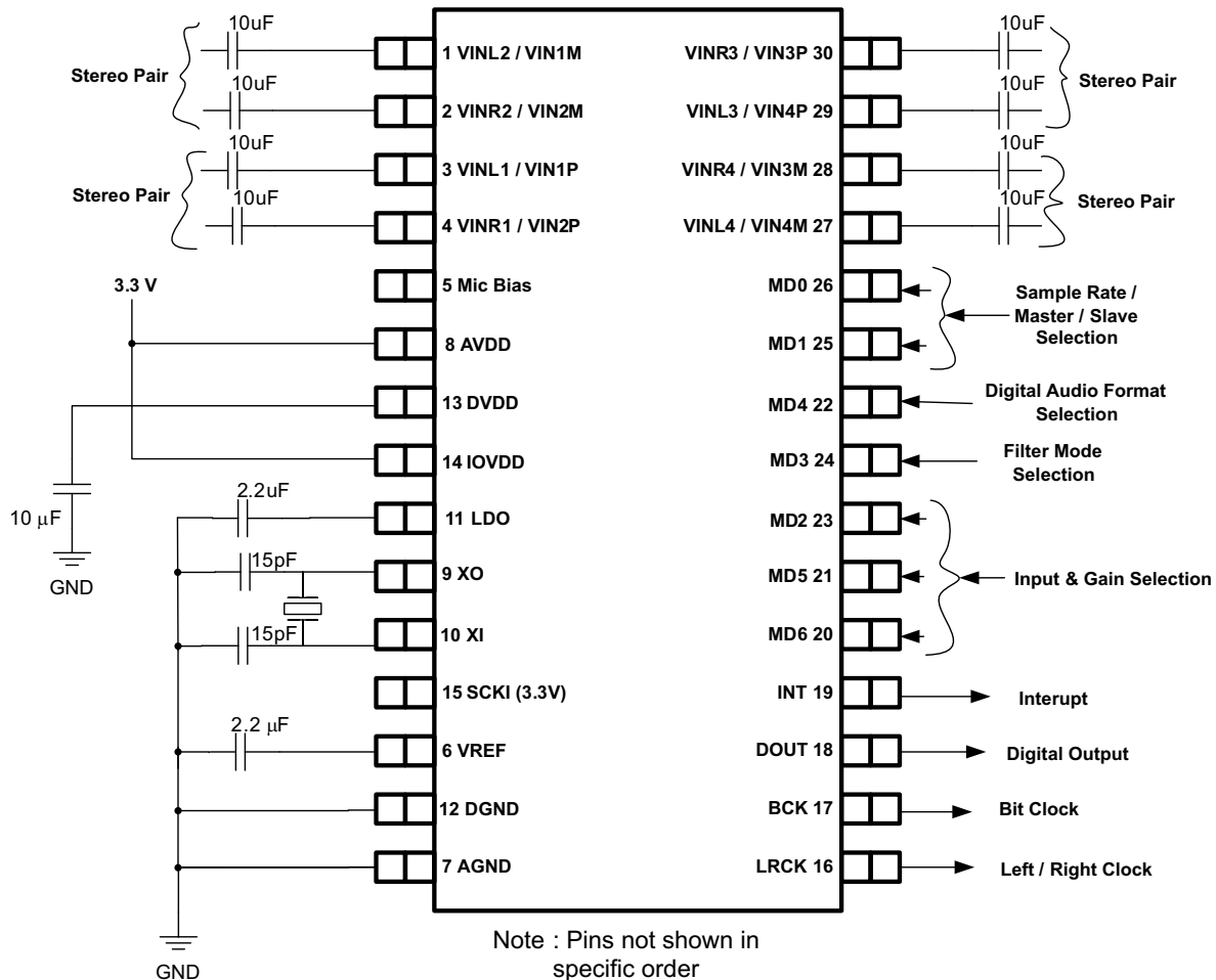
Figure 58. Simplified Schematic, PCM1860 Hardware-Controlled Subsystem
