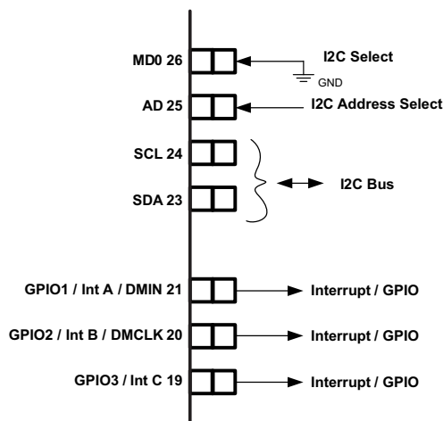
Figure 52. I²C Control Interface Including Interrupt Signals
