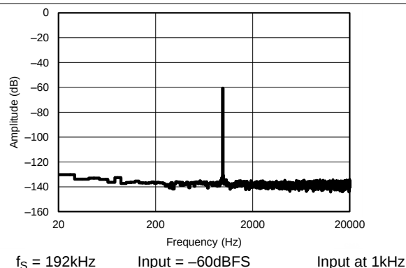
Figure 12. FFT with -60dBFS input
